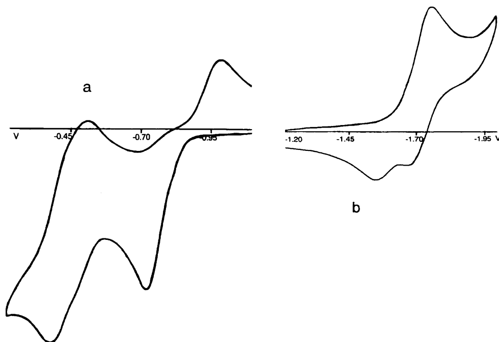
Figure 1. Cyclic voltammograms of a fresh solution 3.0 mM of \text{Co(dppf)}_2 , 1 , in THF, TBAP 0.2 M, at 25 °C, with scan rate 100 mV/s, vs ferrocenium/ferrocene reference: (a) oxidation mode; (b) reduction mode.
